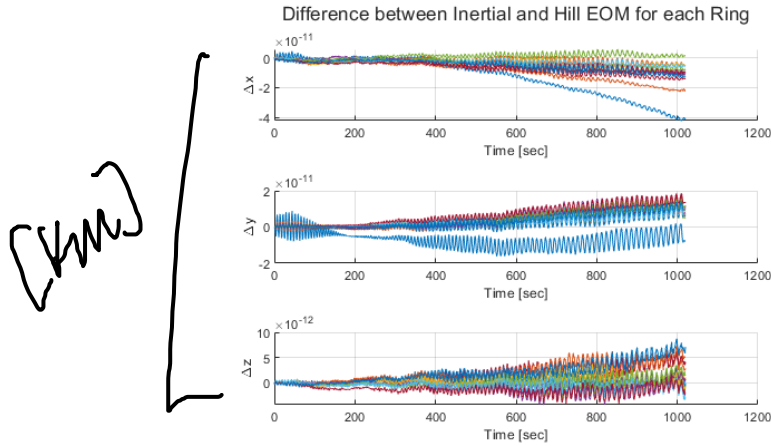
Fig. 11 Difference in Orbit frame and Inertial frame EOM integration, J_2 + drag perturbations
