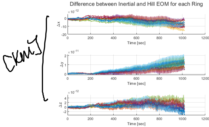
Fig. 7 Difference in Orbit frame and Inertial frame EOM integration, J_2 perturbation only
